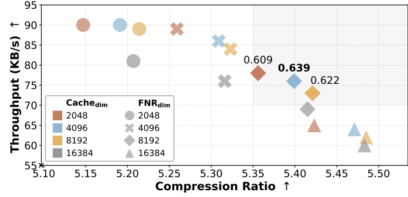
Figure 5: Analysis of different settings on Silesia.
