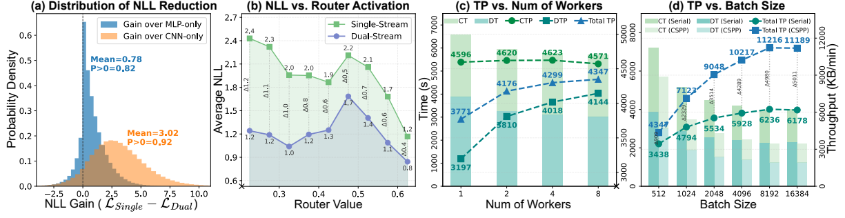
Figure 6: (a-b) NLL characteristics of the dual-stream architecture. (c-d) Impact of worker count and batch size on throughput. CT/DT and CTP/DTP denote Running Time and Throughput of Cmp./Decmp.
